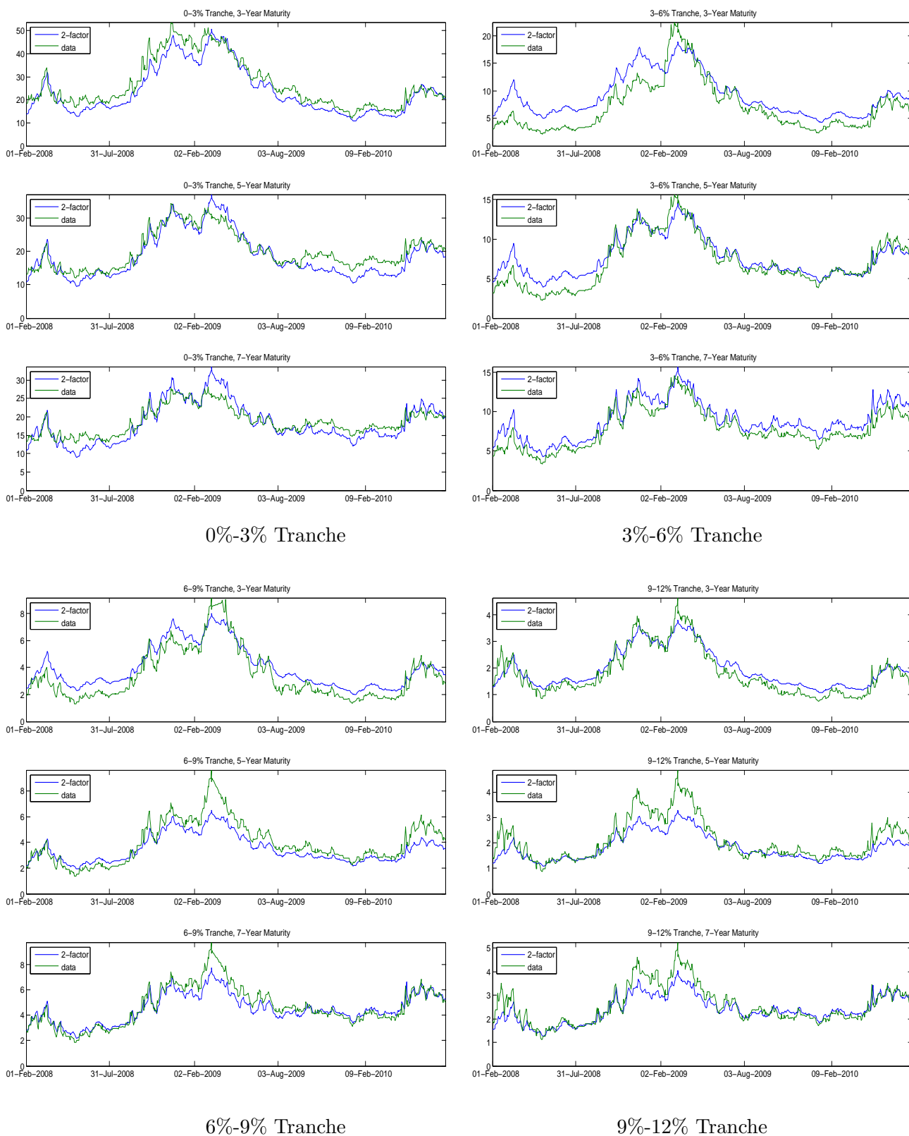
FIGURE 3. Estimated and realized data - part 1.
